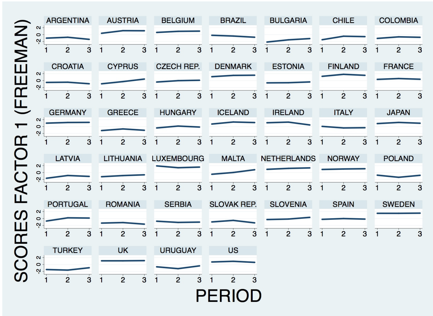
Figure 23: Freeman scores over time by country
